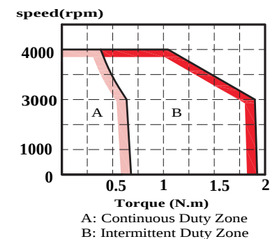
The curve of torque-speed
