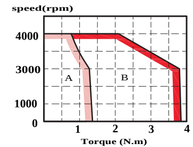
The curve of torque-speed
