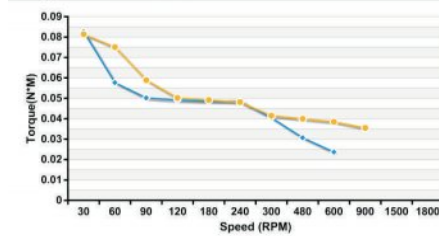
Stepper Motor: 35HS01 (NEMA14, Holding Torque: 0.1 Nm)
