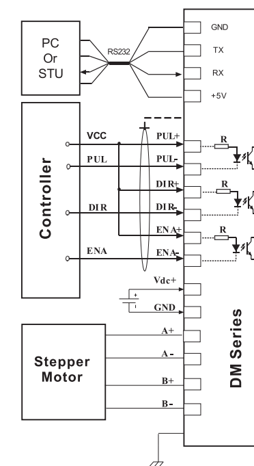
(b) Single-ended (NPN) control signals
