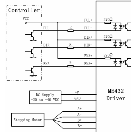
Figure 10: Typical connection
