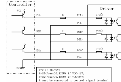
Figure 4: Connection to PNP signal (common-cathode)
