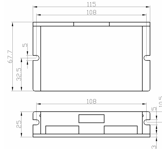
Figure 1: Mechanical specifications
