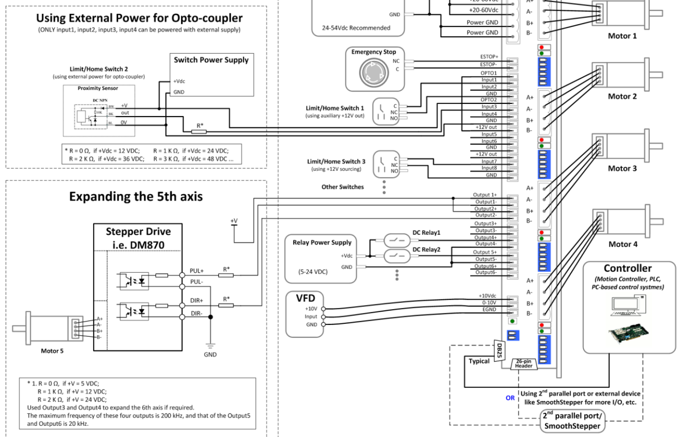
Figure 21 MX4660 Connection Diagram
