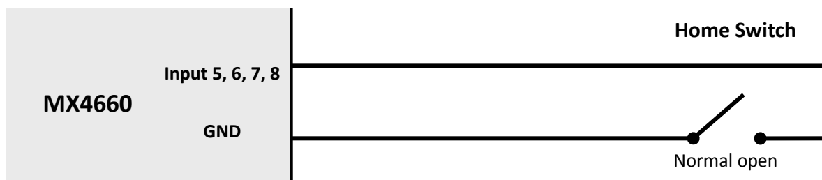
Figure 14 Home / limit switch connections to Input5-8 of the MX4660
