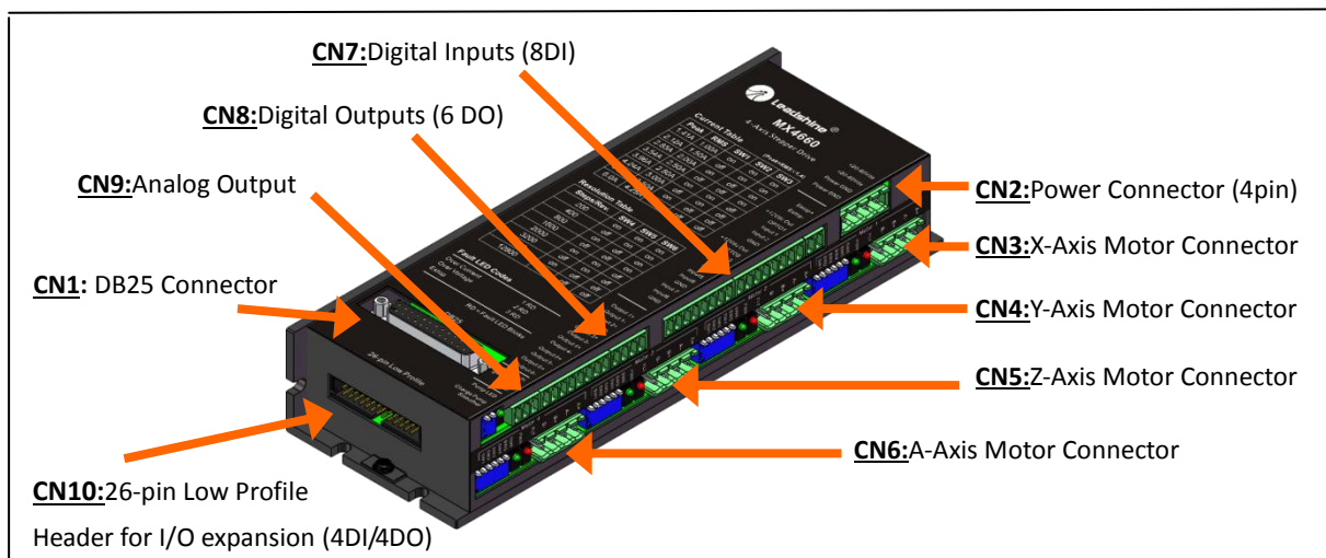
Figure 3 MX4660 layout
