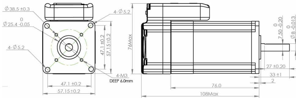
Mechanical Specification of iSV-B23090-01
