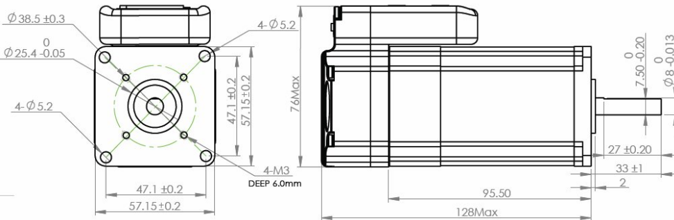
Mechanical Specification of iSV-B23130-01
