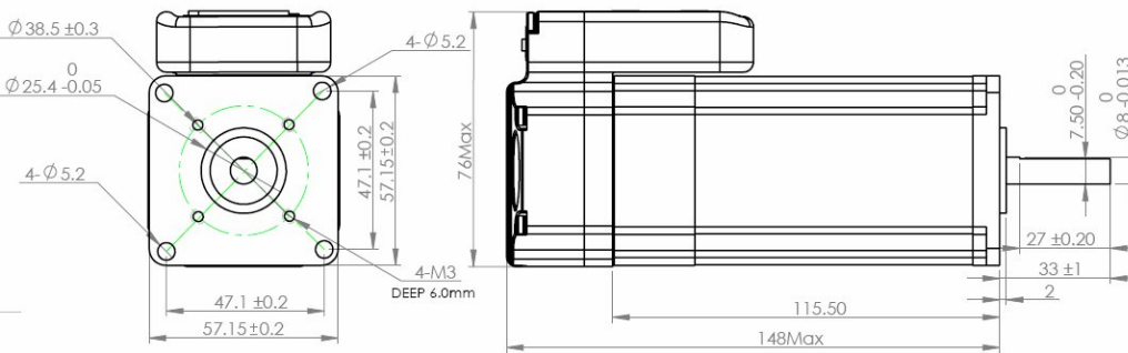
Mechanical Specification of iSV-B23180-01
